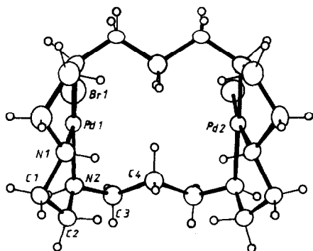
Fig. 7. Molecular structure and the atom-labelling scheme for the \text{Pd}_2([\text{20}] \text{aneN}_6) \cdot \text{Br}_2^+ cation reproduced by permission from ref. 36.
