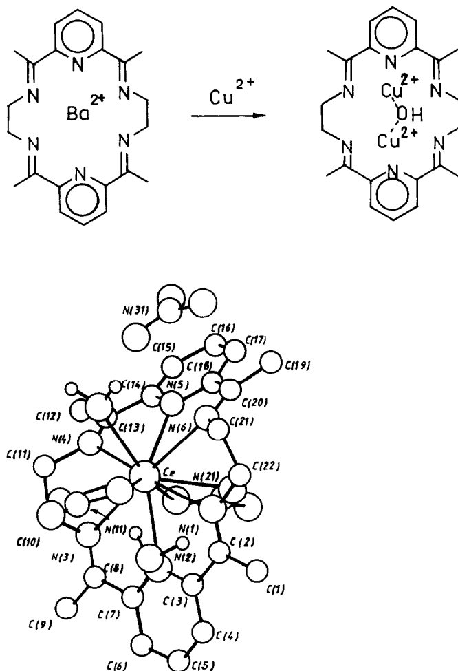
Fig. 16. Molecular structure with atom-labelling scheme for [Ce(L)(NO 3 ) 2 (H 2 O)]NO 3 ·H 2 O (L = XXVI), reproduced by permission from ref. 85.
