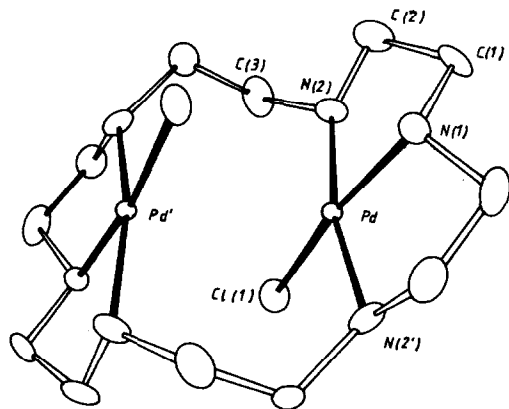
Fig. 2. Molecular structure with the atom-labelling scheme for the complexed cation [(\text{Pd}_2-[\text{18}] \text{aneN}_6)\text{Cl}_2]^+ reproduced by permission from ref. 35(a).
