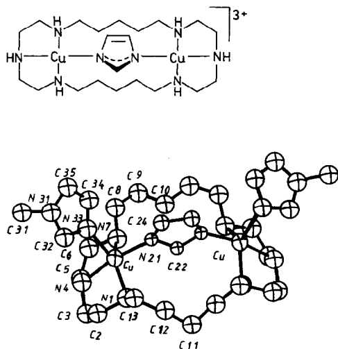
Fig. 8. Molecular structure and the atom-labelling scheme for [\text{Cu}_2(\text{im})(\text{Meim})_2\text{L}]^{3+} ( \text{L} = 1,4,7,13,16,19\text{-hexaazacyclotetrasane} , \text{im} = \text{imidazole} , \text{Meim} = \text{methylimidazole} ), reproduced by permission from ref. 42.
