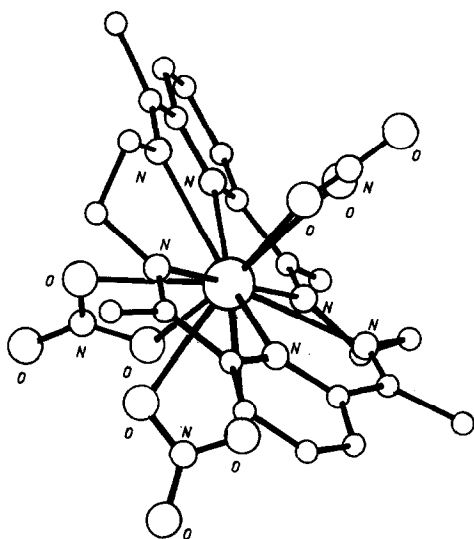
Fig. 13. Molecular structure and atom-labelling scheme for [\text{La}(\text{L})](\text{NO}_3)_3 ( \text{L}=\text{XXVI} ) reproduced by permission from ref. 76.
