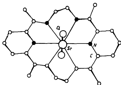
Fig. 12. Molecular structure and atom-labelling scheme for \text{Sr}(\text{L})\text{Cl}_2 ( \text{L}=\text{XXVI} ) reproduced by permission from ref. 75.
